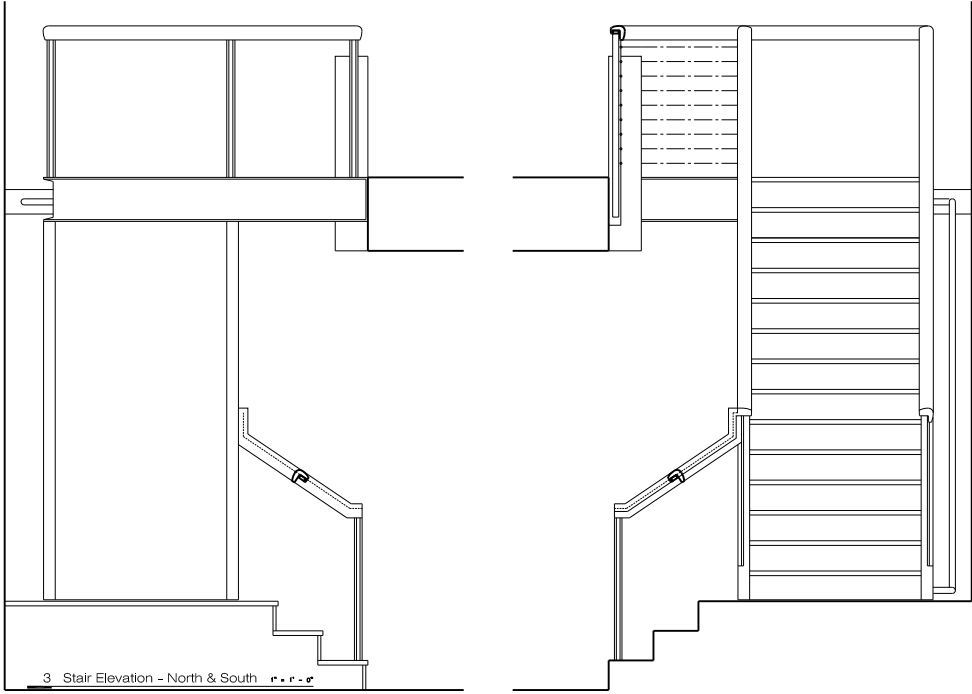
3 Stair Elevation - North & South r • r - g
